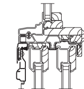
Direct Glaze Transom Over Sliding Patio Door
